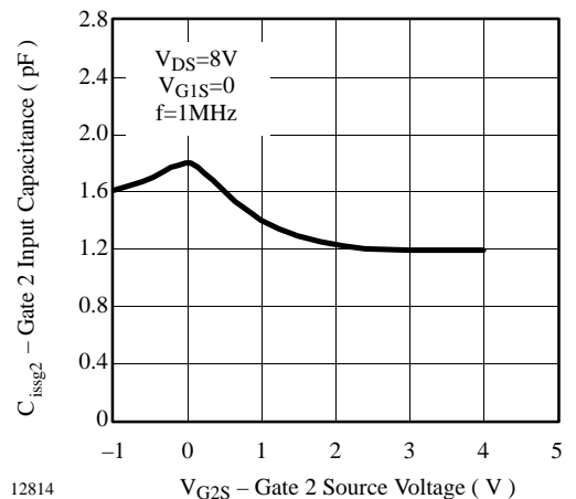
Figure 6. Gate 2 Input Capacitance vs. Gate 2 Source Voltage
